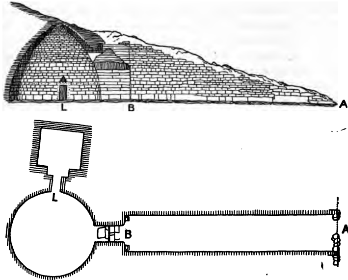
FIG. 57.— SECTION AND PLAN OF DOMED TOMB (Tholos) AT MYCENÆ
